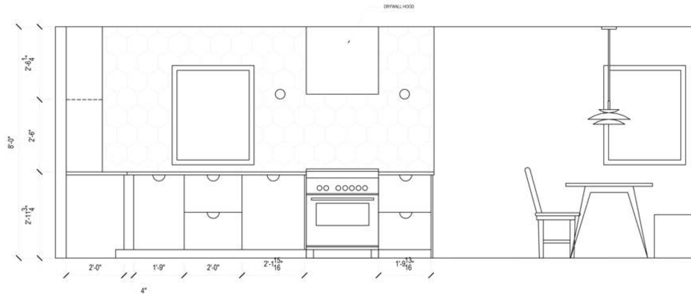
RANGE WALL ELEVATION
