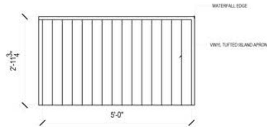
ISLAND ELEVATION BACK
