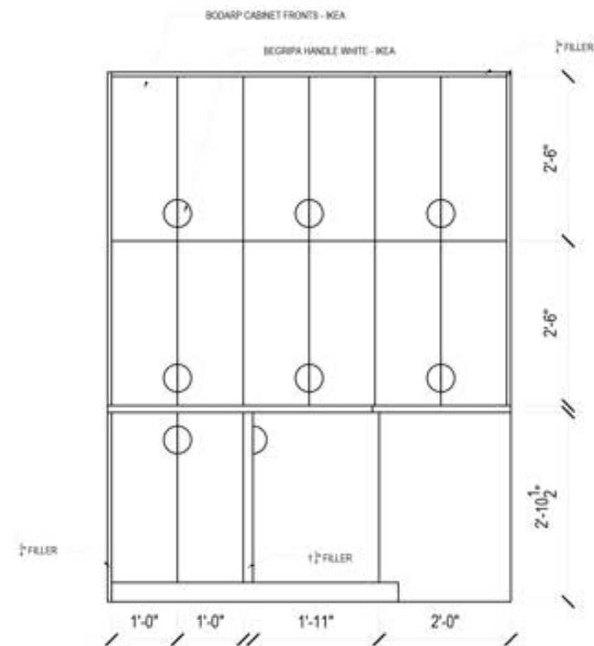
PANTRY WALL ELEVATION
