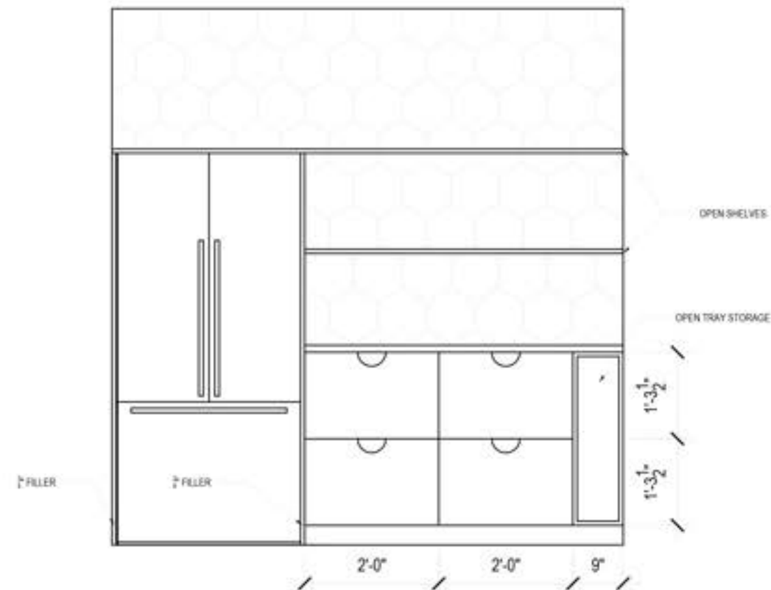
FRIDGE NOOK ELEVATION
