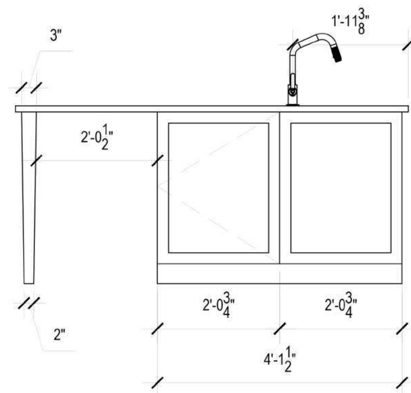
ISLAND RIGHT ELEVATION
