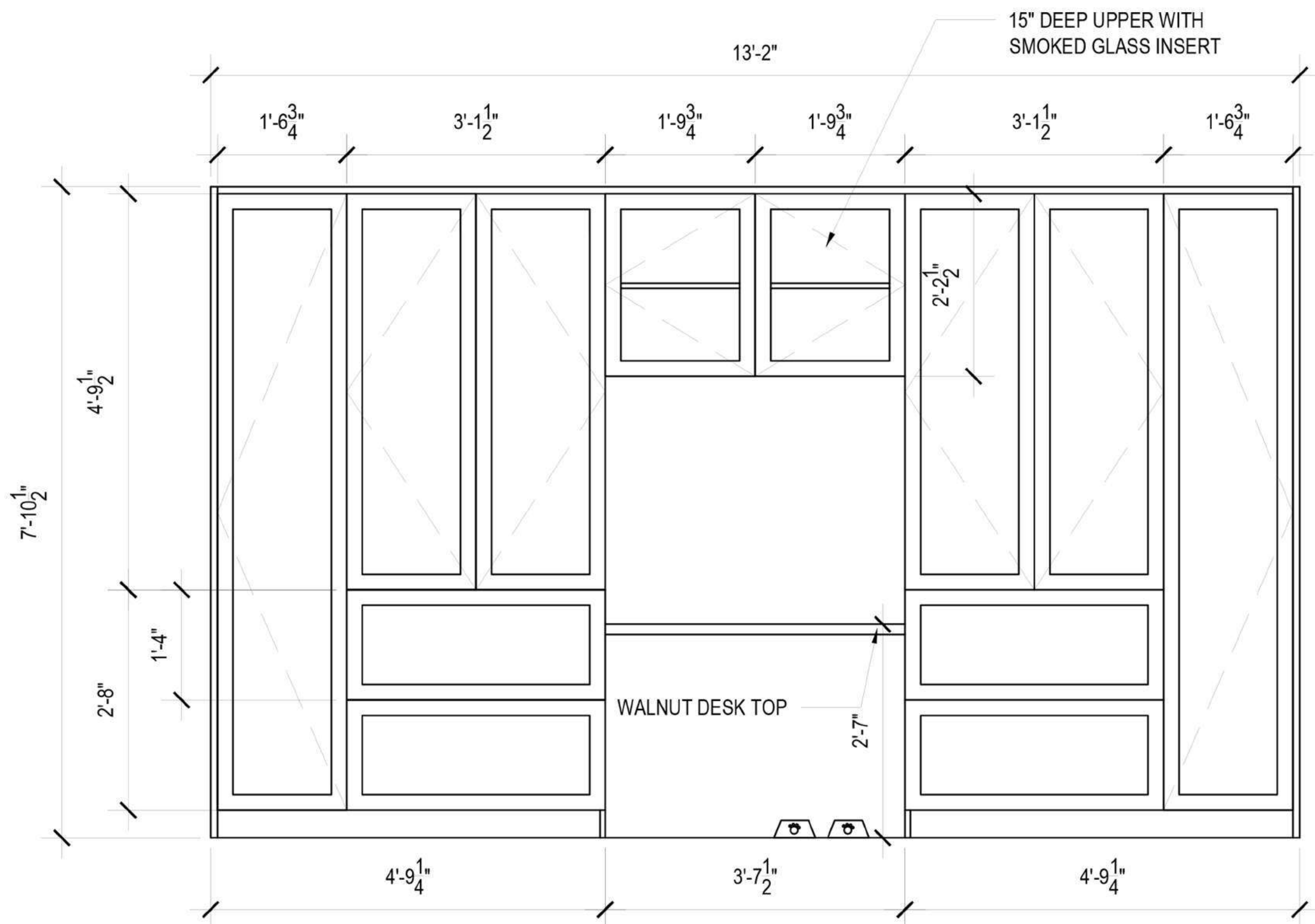
PANTRY WALL ELEVATION EXTERIOR
