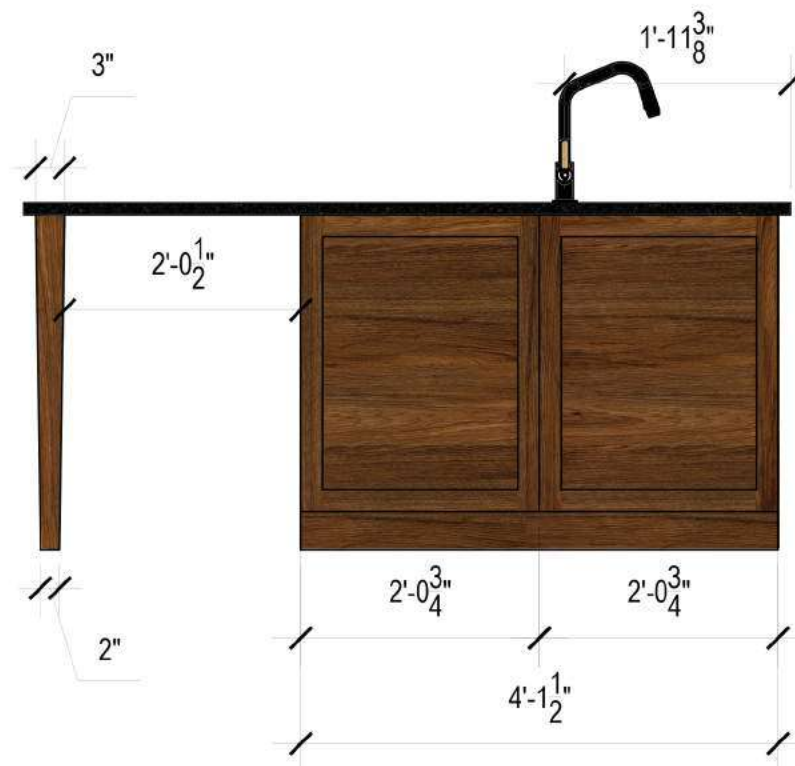
ISLAND RIGHT ELEVATION
