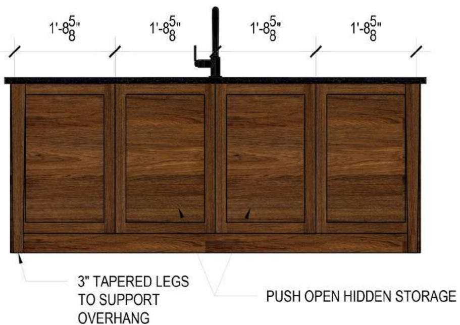
ISLAND FRONT ELEVATION
