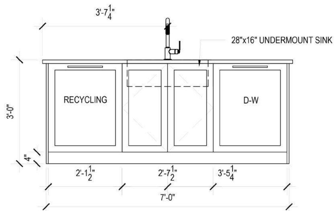
ISLAND BACK ELEVATION
